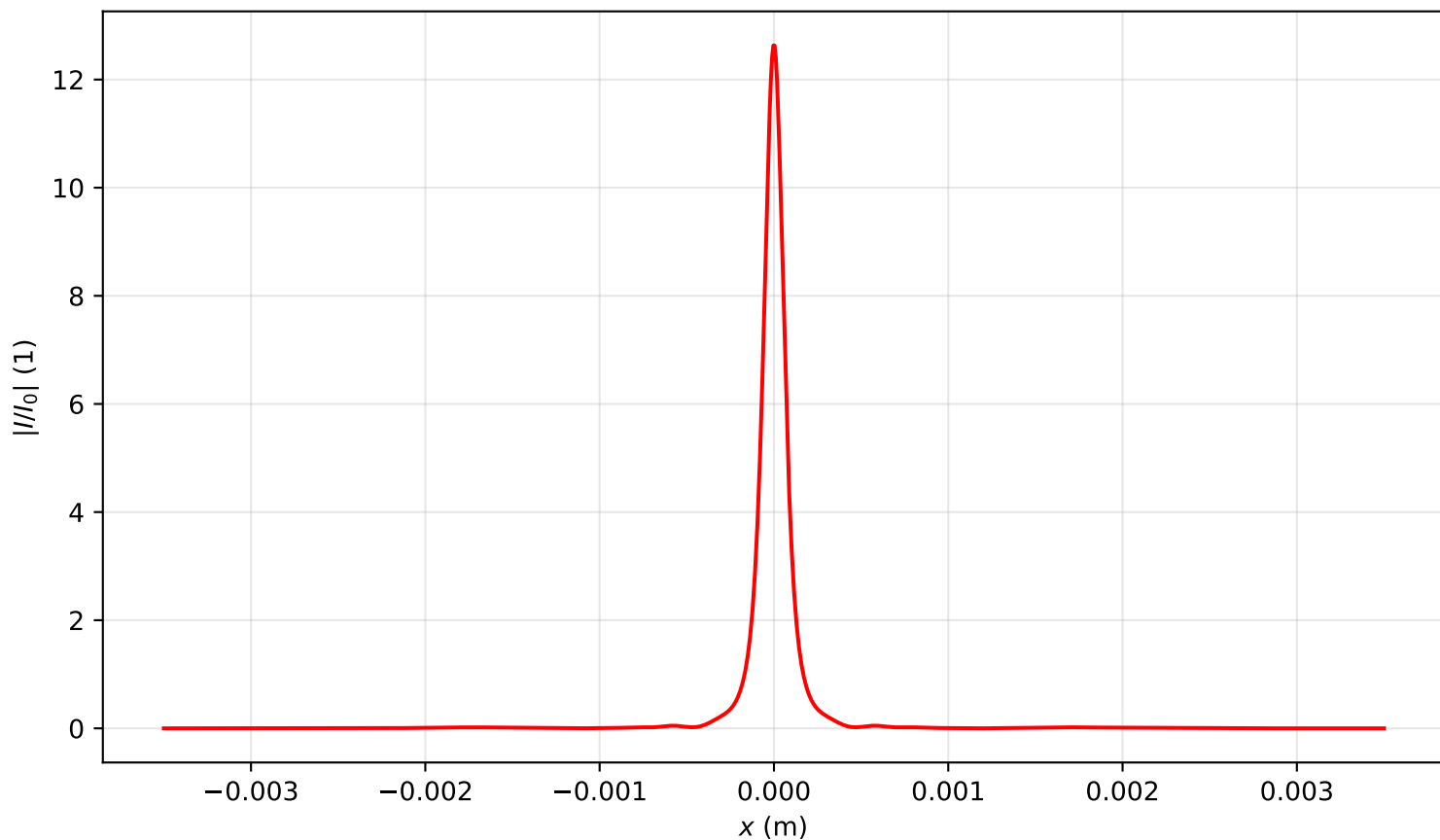
Intensity profile I(x, y = 0, z = 2.866)/I_0 , P_{in}=2.0P_{cr} , artificial time
